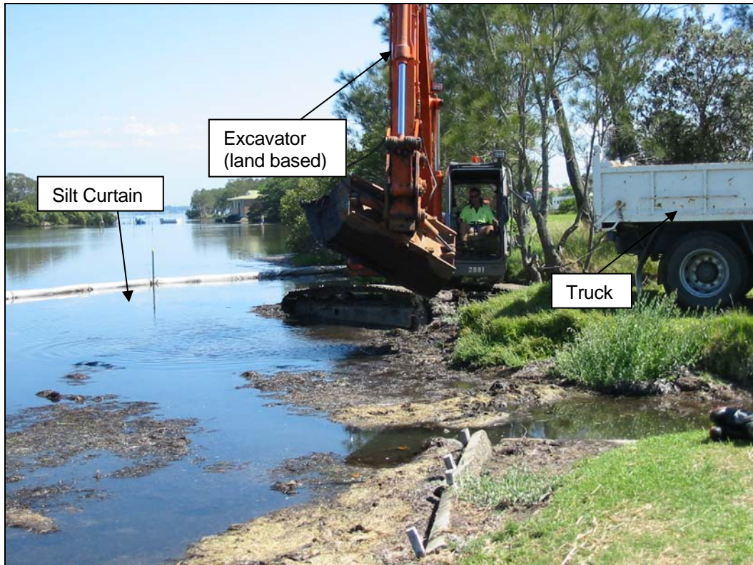
Figure 2.10 Removal of Sediment from Stormwater Channel Entrance
