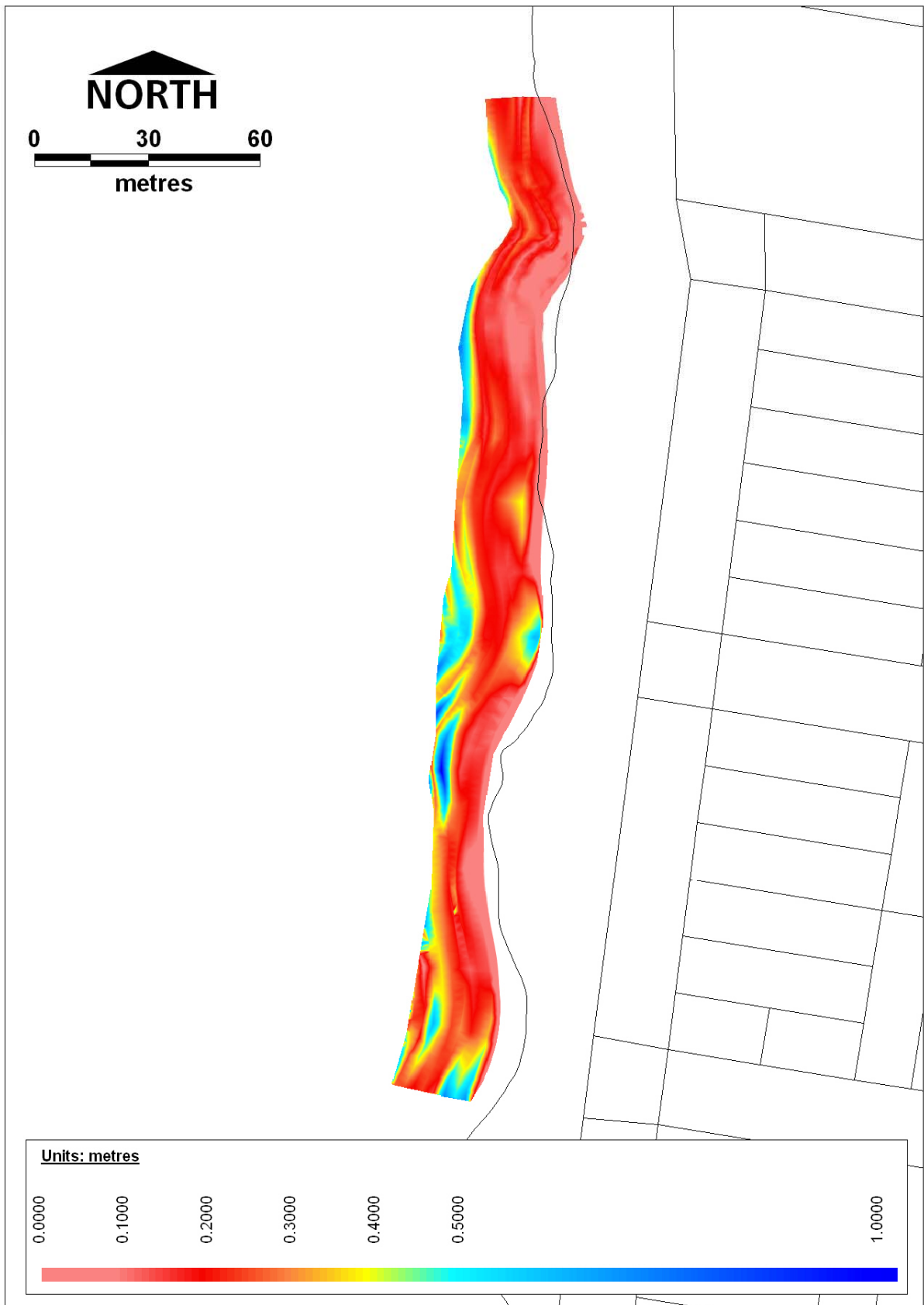
Figure 2.2 Depth of unconsolidated (organic) sediment at Swansea Flats (derived from survey by Cadman Consultants, 2004)
