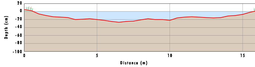
Channel Profile - Island 2 to Island 3
