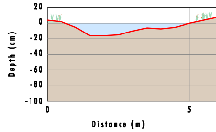
Channel Profile - Island 3 to Island 4
